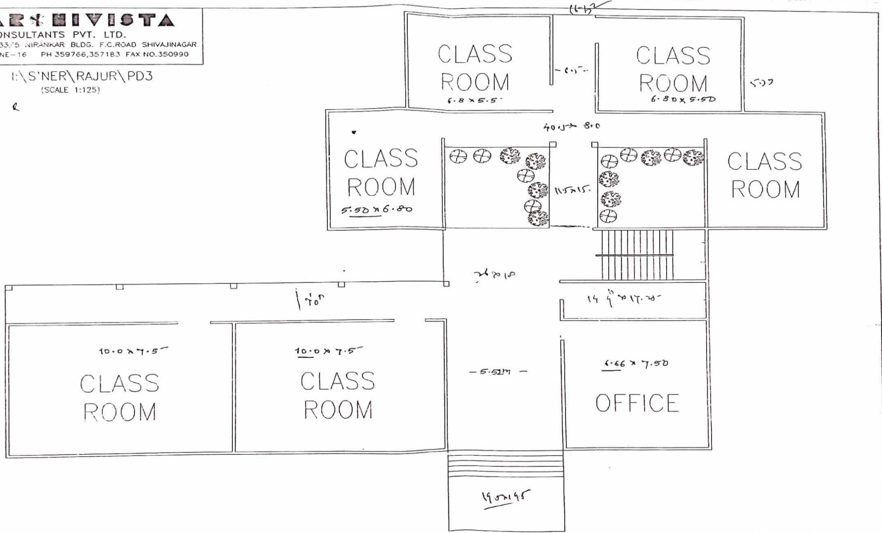
PROPOSED BLDG. FOR ART FACULTY FOR SATYANIKETAN SANSTHA AT RAJUR
